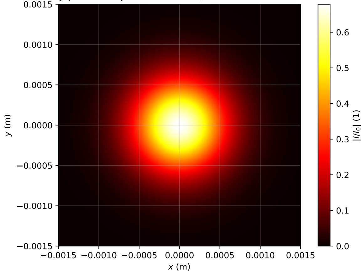
Intensity profile I(x, y, z = 1.911m)/I_0 , \text{Pin}=0.3\text{Pcr} , artificial time
